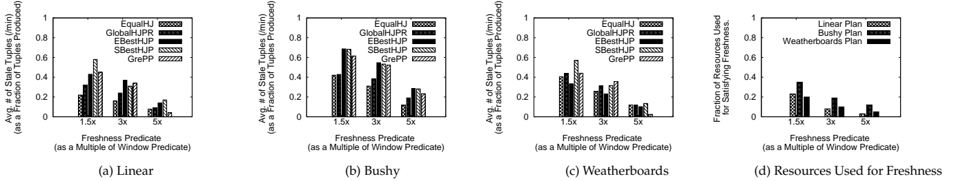
Fig. 9. Evaluation of freshness predicates.
