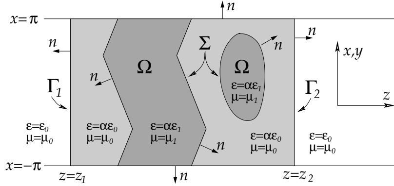
Figure 2: A two-dimensional depiction of one period of a possible augmented three-dimensional slab structure.
