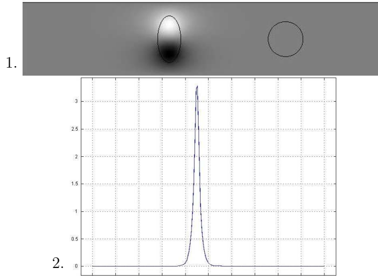
Figure 4: 1. Eigenfunction for the first real eigenvalue \epsilon_1 \approx 9.762 for the parameters \omega = 1, \epsilon_0 = 1, \mu_0 = \mu_1 = 1, \kappa = (0, 0) . 2. Cross section of the solution along the line z = \pi/2 ; the magnitude of the solution is plotted.
