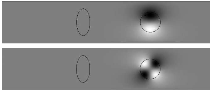
Figure 5: Eigenfunctions for the second and third real eigenvalues \epsilon_1 \approx 11.00 and \epsilon_1 \approx 25.66 for the parameters \omega = 1, \epsilon_0 = 1, \mu_0 = \mu_1 = 1, \kappa_1 = 0 . These are nonrobust guided modes.
