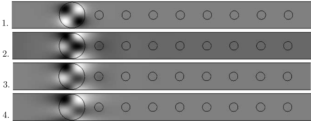
Figure 3: Four guided modes in a two-dimensional structure investigated in [2] (Fig. 7.2). One period is shown; the structure continues periodically in the vertical direction on the page. 1. A nonrobust antisymmetric guided mode at Bloch wavevector zero, (\kappa_1, \omega) = (0.0, 0.4017) . 2 and 3. Nonrobust guided modes at nonzero wavenumbers in the direction perpendicular to the line of symmetry, (\kappa_1, \omega) = (0.14, 0.3863), (0.22, 0.3707) . 4. A robust guided mode, (\kappa_1, \omega) = (0.44, 0.3306) .
