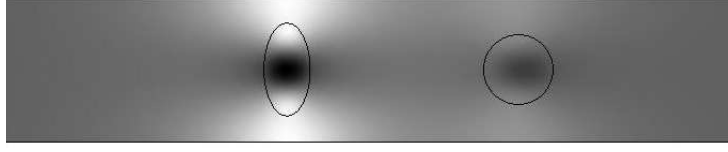
Figure 6: Eigenfunction for the third real eigenvalue \epsilon_1 \approx 11.42 for the parameters \omega = 0.3, \epsilon_0 = 1, \mu_0 = 1, \mu_1 = 3, \kappa_1 = 0.4 . This is a robust guided mode.
