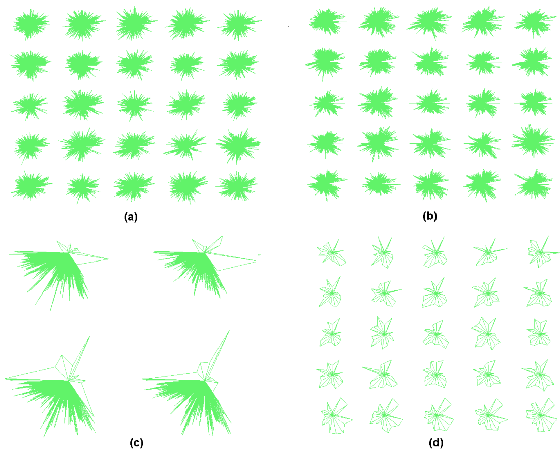
Figure 3: Star Glyphs. (a): OHSUMED dataset without DOSFA. (b): after ordering and spacing. (c): distorted star glyphs. (d): after filtering.
