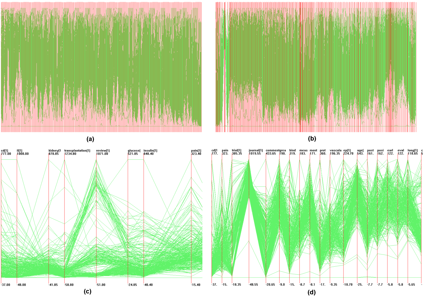
Figure 2: Parallel Coordinates. (a): OHSUMED dataset without DOSFA. (b): after ordering and spacing. (c): after zooming. (d): after filtering.
