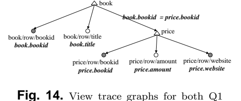
Fig. 14. View trace graphs for both Q1 and Q2
