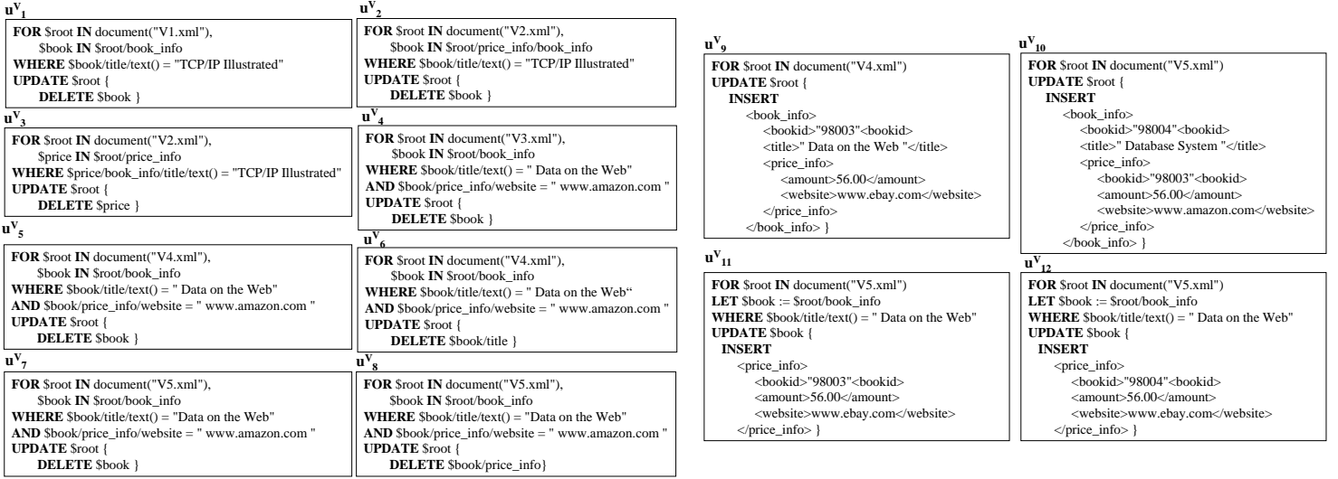
Fig. 5. Update operations on XML views defined in Fig.4
