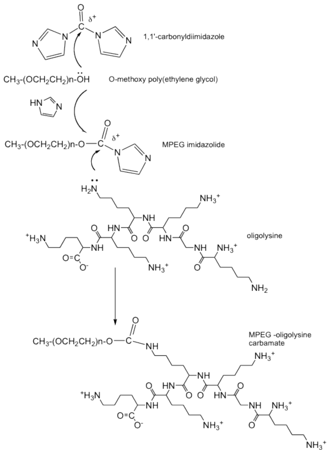
Figure 5: A scheme of MPEG-Imidazolide synthesis and its reaction with pentalysine (illustrating a fragment Poly-L-Lysine)
