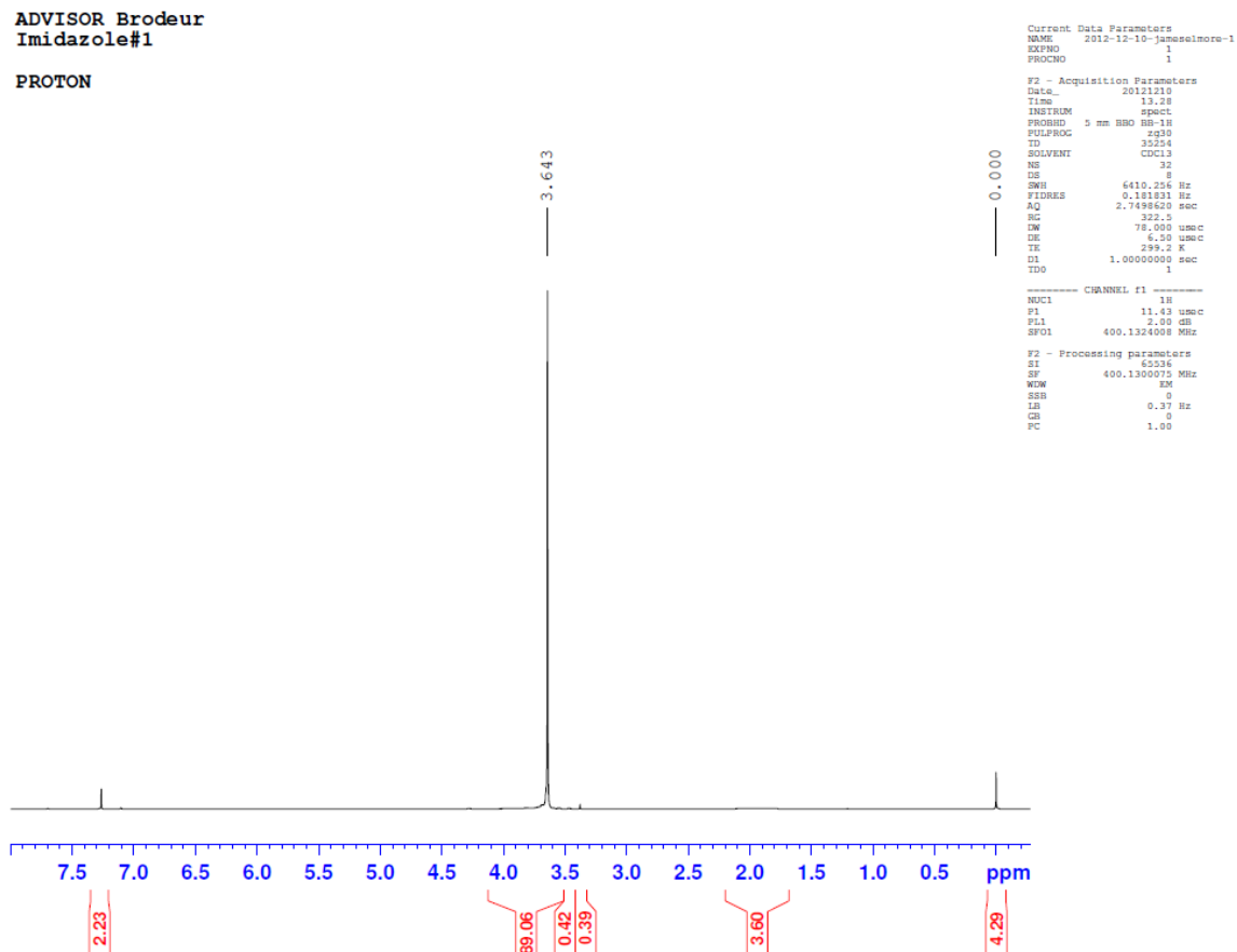
Figure 7: NMR Spectrum of MPEG-Imidazolide Sample 1
