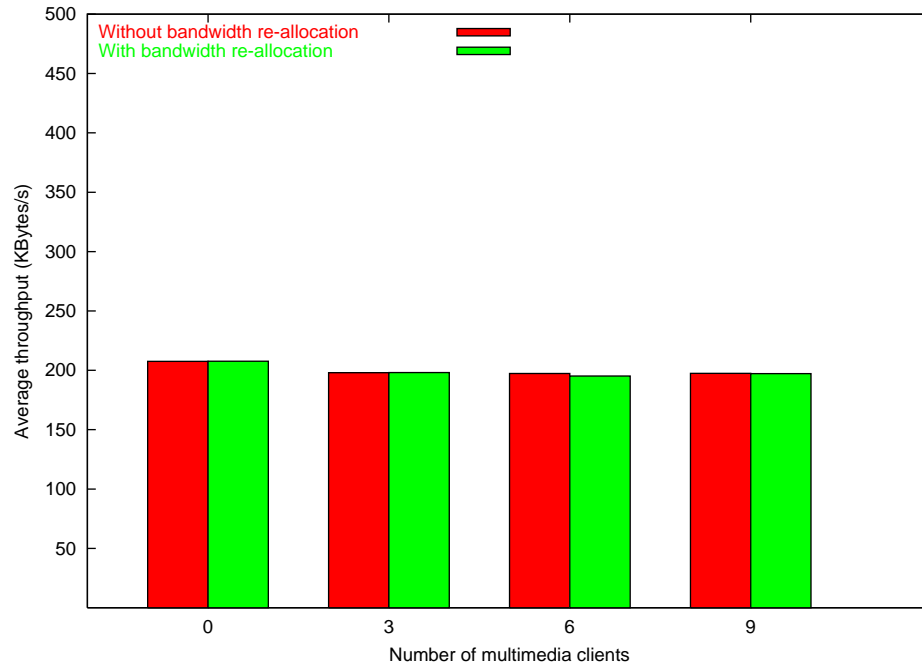
Figure 5.25: Average throughput with and without bandwidth re-allocation policies under Clarity when non-multimedia service class is under-utilized
