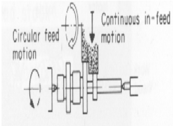
Figure 2.5 OD grinding
