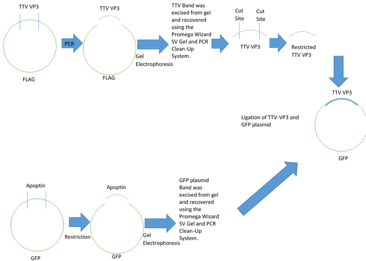
FIGURE 6: TTV VP3 GFP CONSTRUCT DESIGN SCHEMATIC
