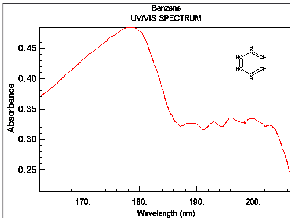
(UV/VIS Absorption Spectrum of benzene)
