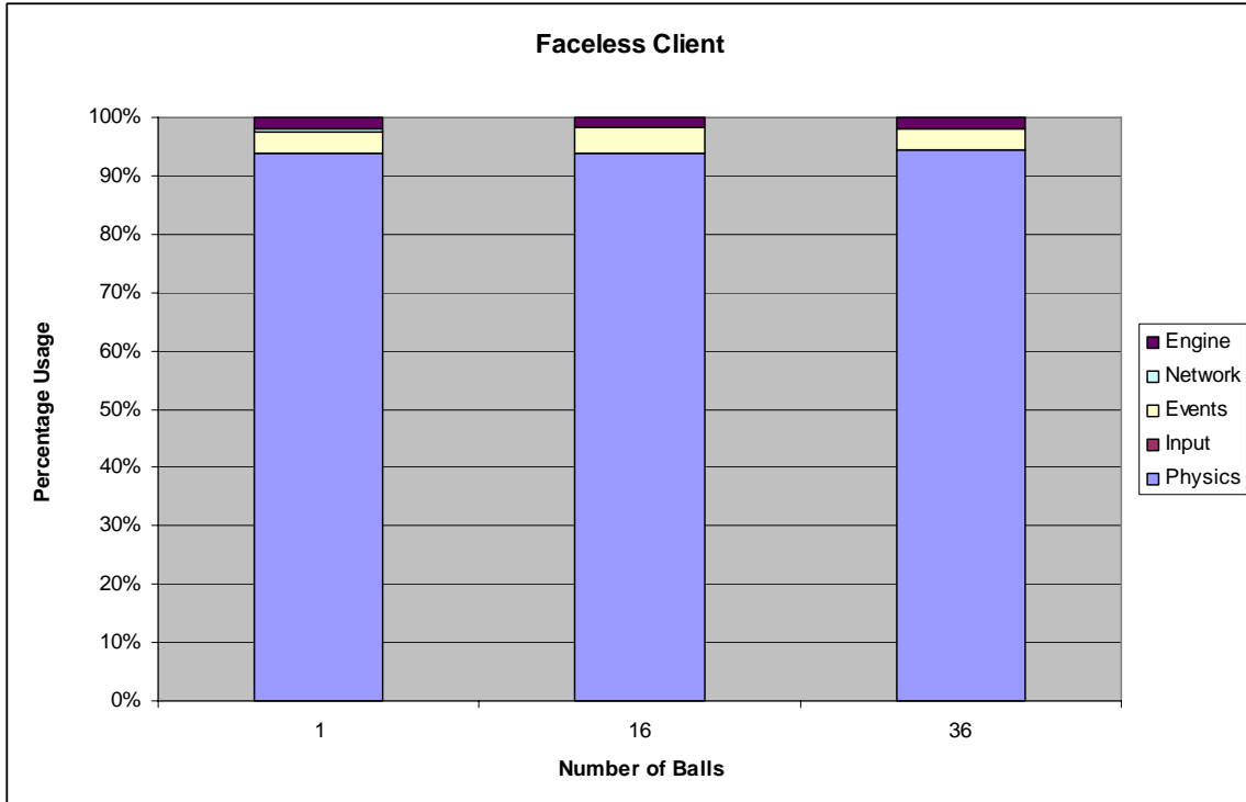
Figure 7.5.2-1: Client Workload Breakdown vs. Number of Balls (faceless)
