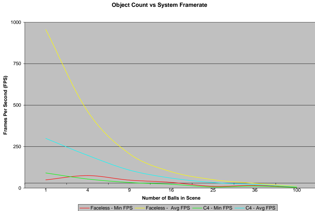
Figure 7.3-1: Client System Framerate vs. Objects Count
