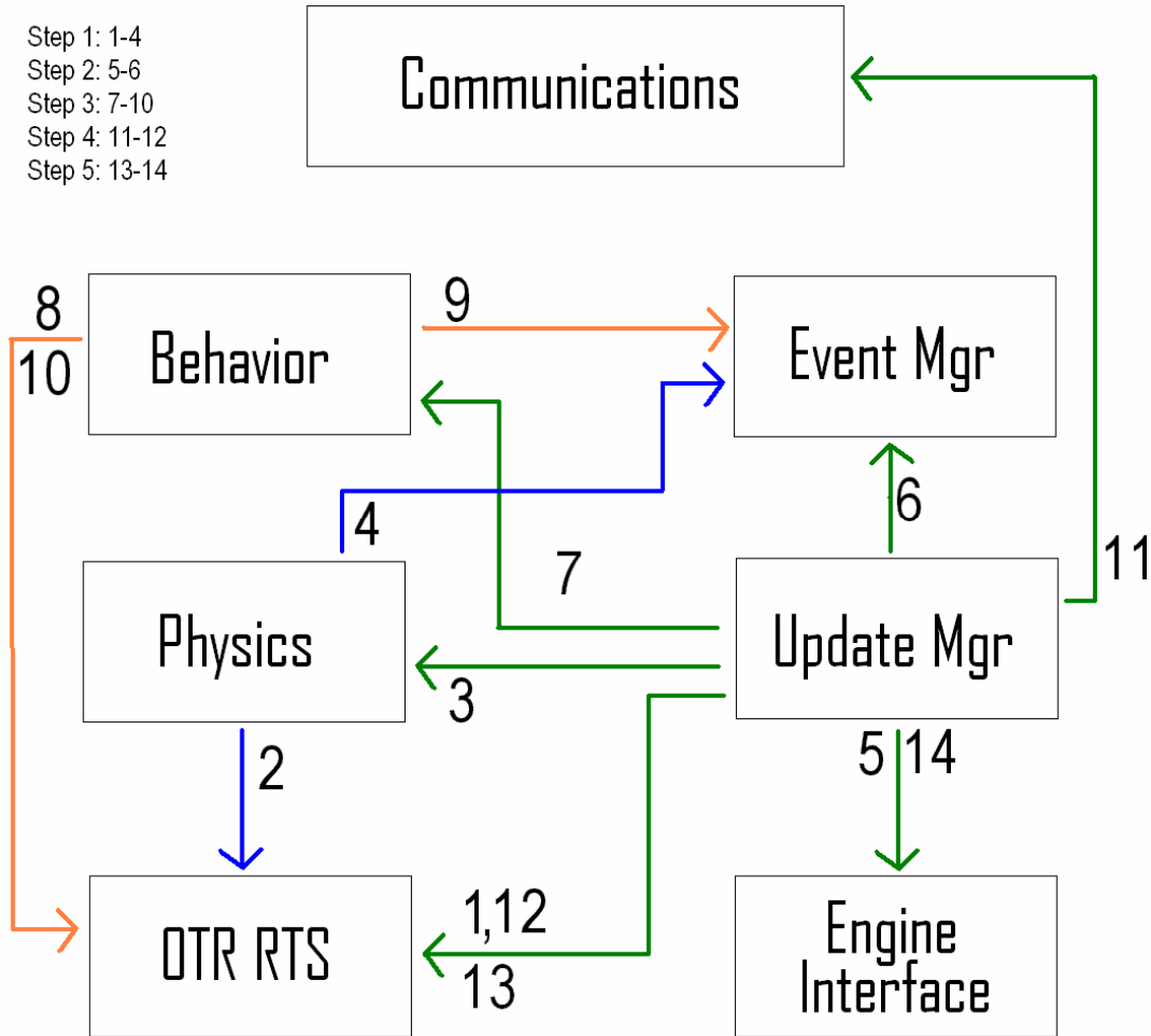
Figure 6.4.9-1: Processing a time slice.
