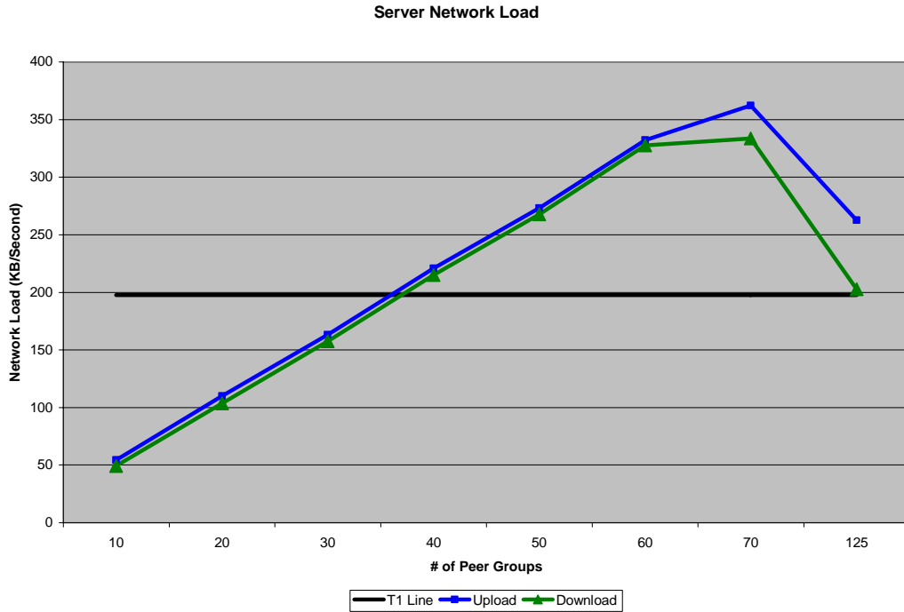
Figure 7.4-2: Server bandwidth
