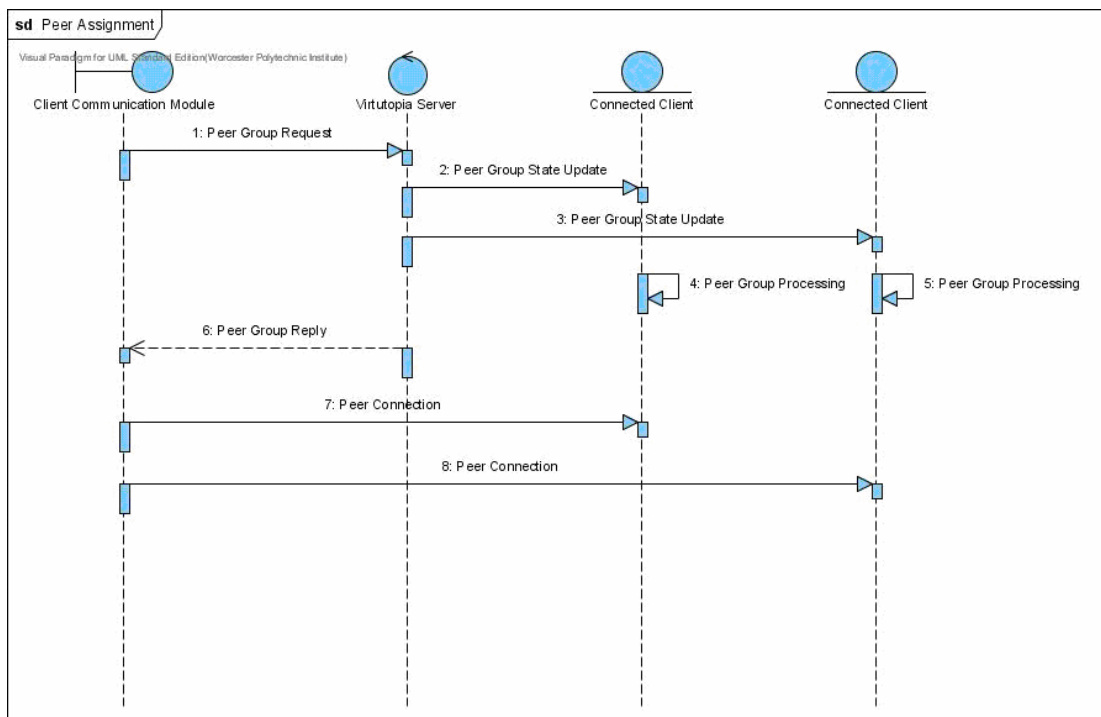
Figure 6.5.1-2 1 Virtutopia Peer Assignment
