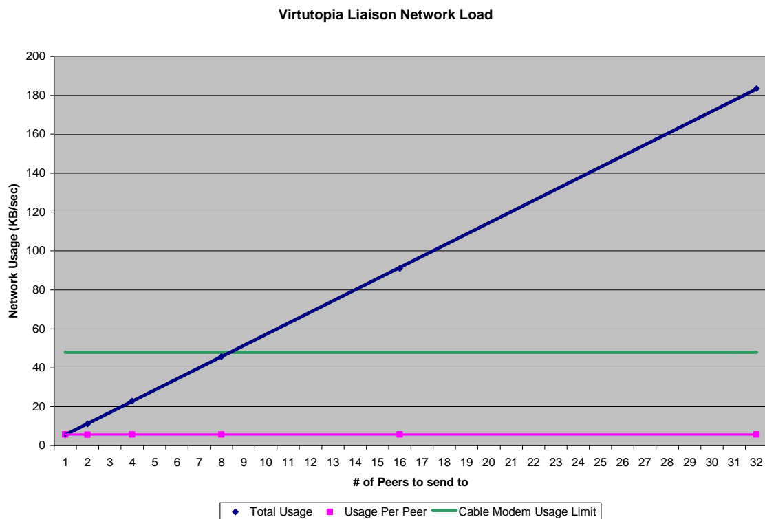
Figure 7.2-1: Virtutopia Liaison Network Load vs. Peer Group Size
