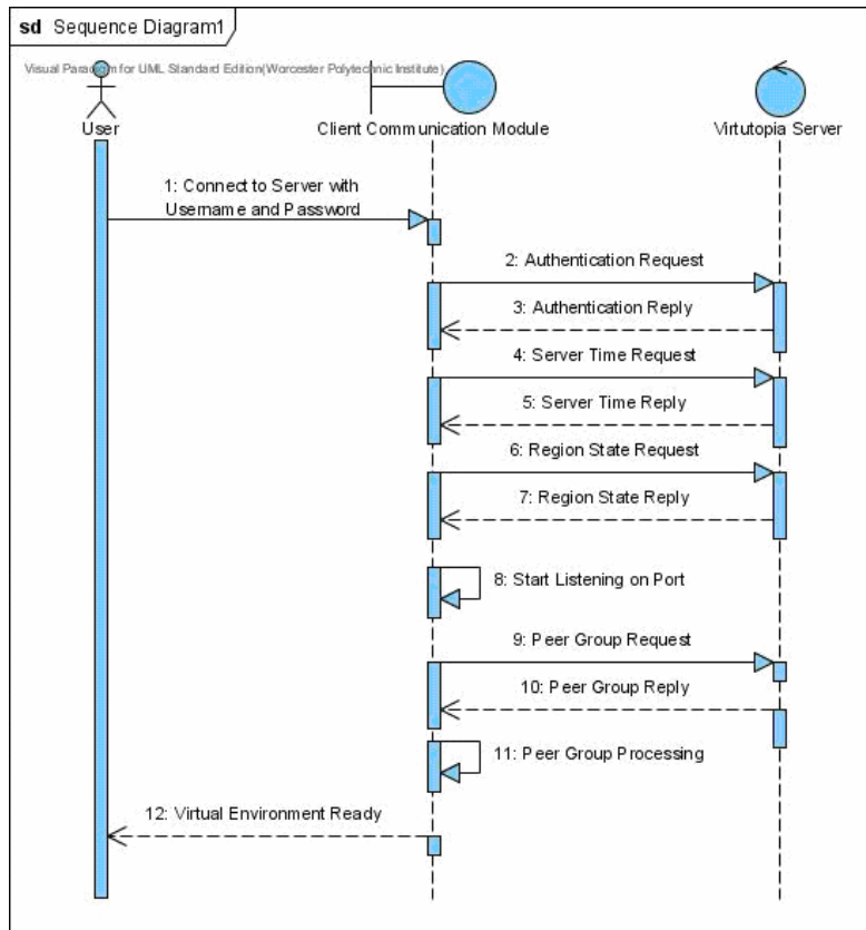
Figure 6.5.1-1: Virtutopia Connection Process
