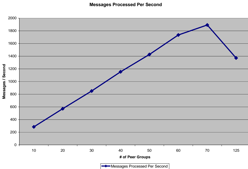
Figure 7.4-1: Server-processed messages per second
