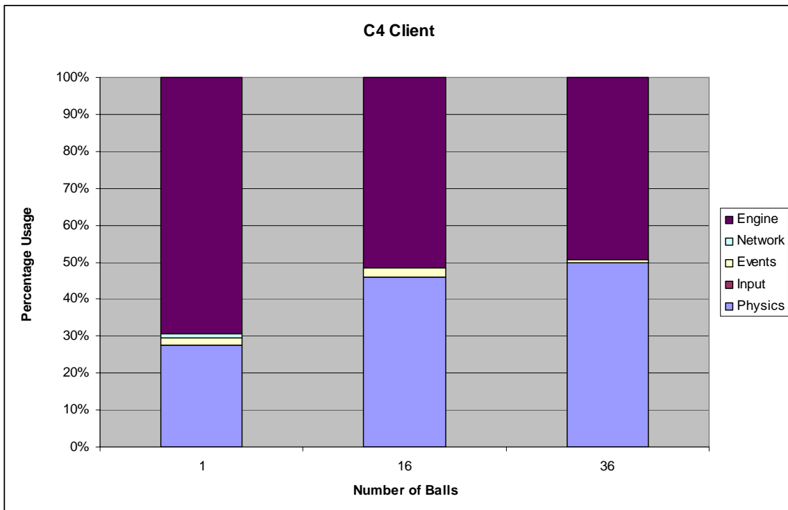
Figure 7.5.2-2: Client Workload Breakdown vs. Number of Balls (C4)
