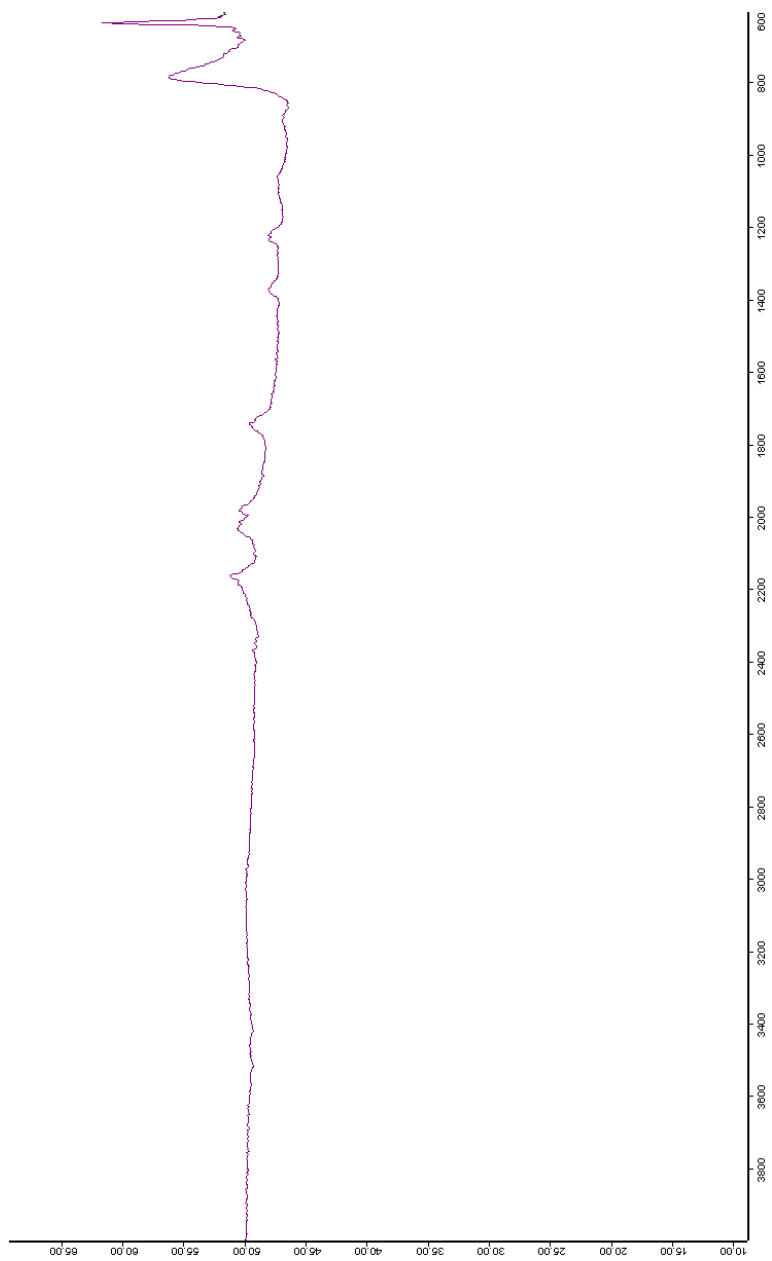
Figure 33 - Copper bromide
