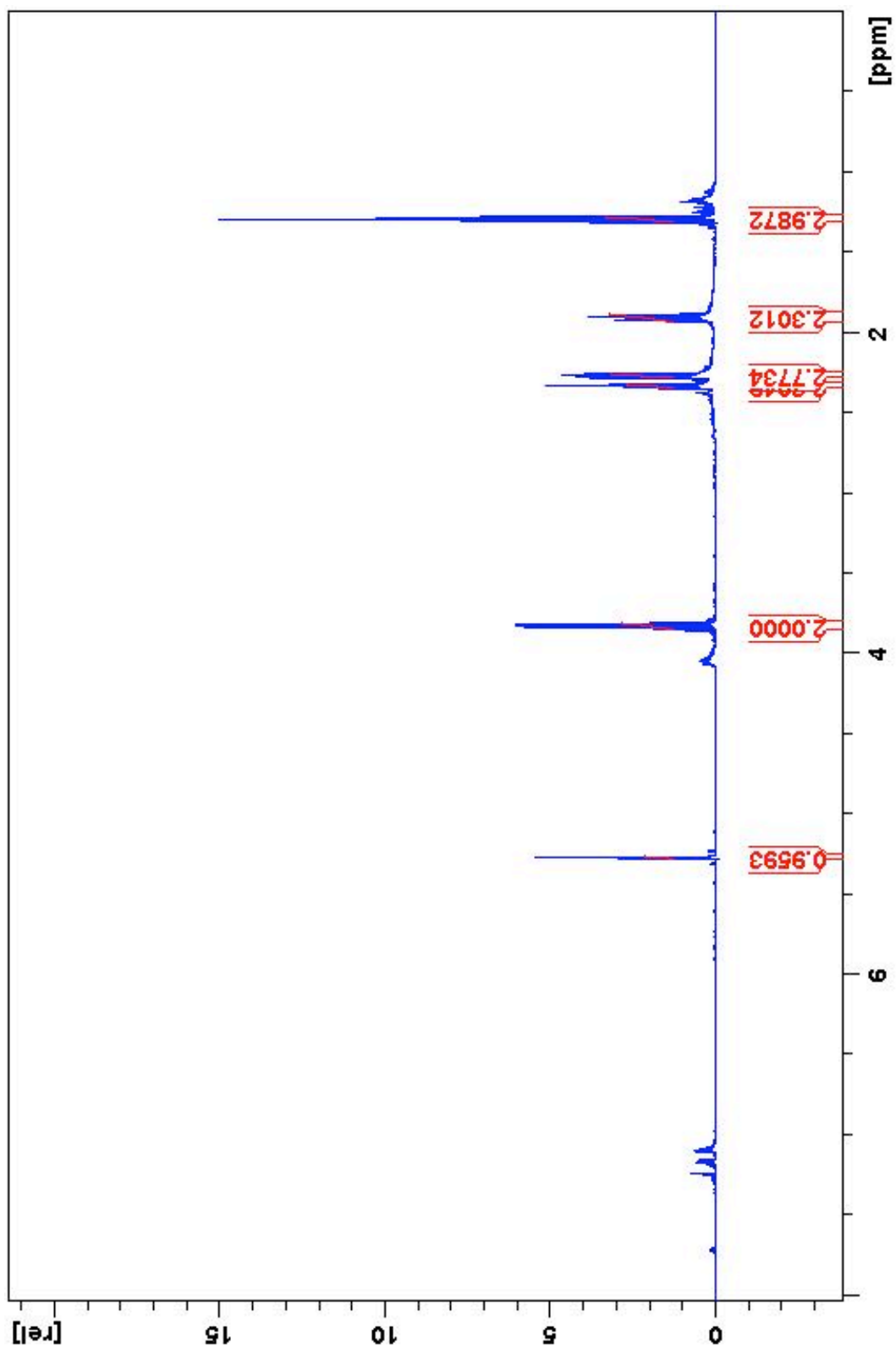
Figure 10: ^1\text{H} NMR 3-ethoxy-3-cyclohexenone (BCC-i-001c)
