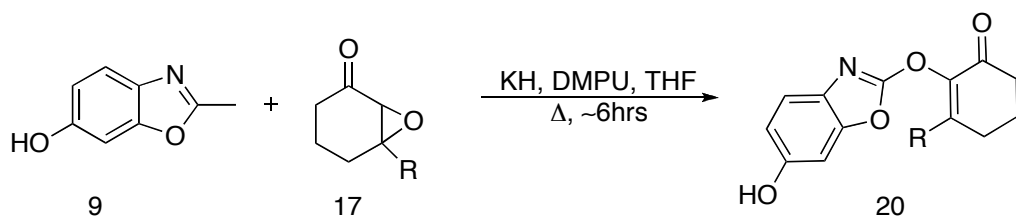
Figure 9: Synthetic route for the production of 3-(but-3-enyl)-2-(2-methylbenzo[d]oxazol-6-yloxy)cyclohex-2-enone
