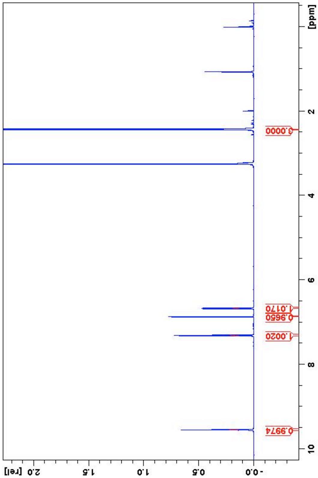
Figure 14: 1 H NMR 2-methylbenzo[d]oxazol-6-ol (AEV-I-021)
