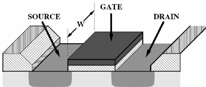
Figure 6. Gate Oxide 43 .
