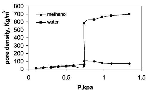
FIG. 13. Pore densities of methanol and water as a function of bulk pressure for 50–50 mole % mixture of methanol-water in 15 Å pore width at 298 K.
