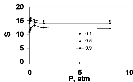
FIG. 6. Selectivity of ethane over methane as a function of operating pressure for 10 Å pore size at 280 K. Results shown for y_{b1}=0.9, 0.5, and 0.1 (methane).
