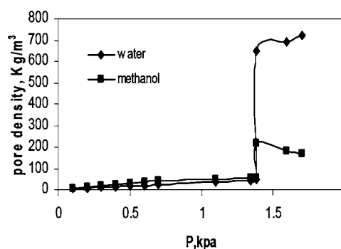
FIG. 15. Pore densities of methanol and water as a function of bulk pressure for 50–50 mole % mixture of methanol-water in 25 Å pore width at 298 K.
