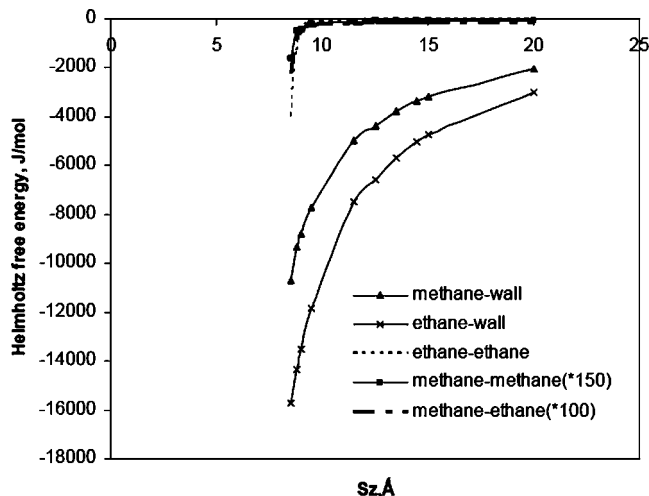
FIG. 2. Relative magnitudes of methane-wall, ethane-wall, ethane-ethane, methane-methane ( \times 150 ), and methane-ethane ( \times 100 ) interactions as a function of pore width for y_{b1}=0.9 (methane) at 280 K.
