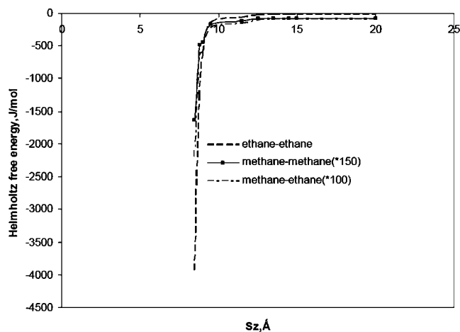
FIG. 3. Relative magnitudes of ethane-ethane, methane-methane ( \times 150 ), and methane-ethane ( \times 100 ) interactions as a function of pore width for y_{b1}=0.9 (methane) at 280 K.
